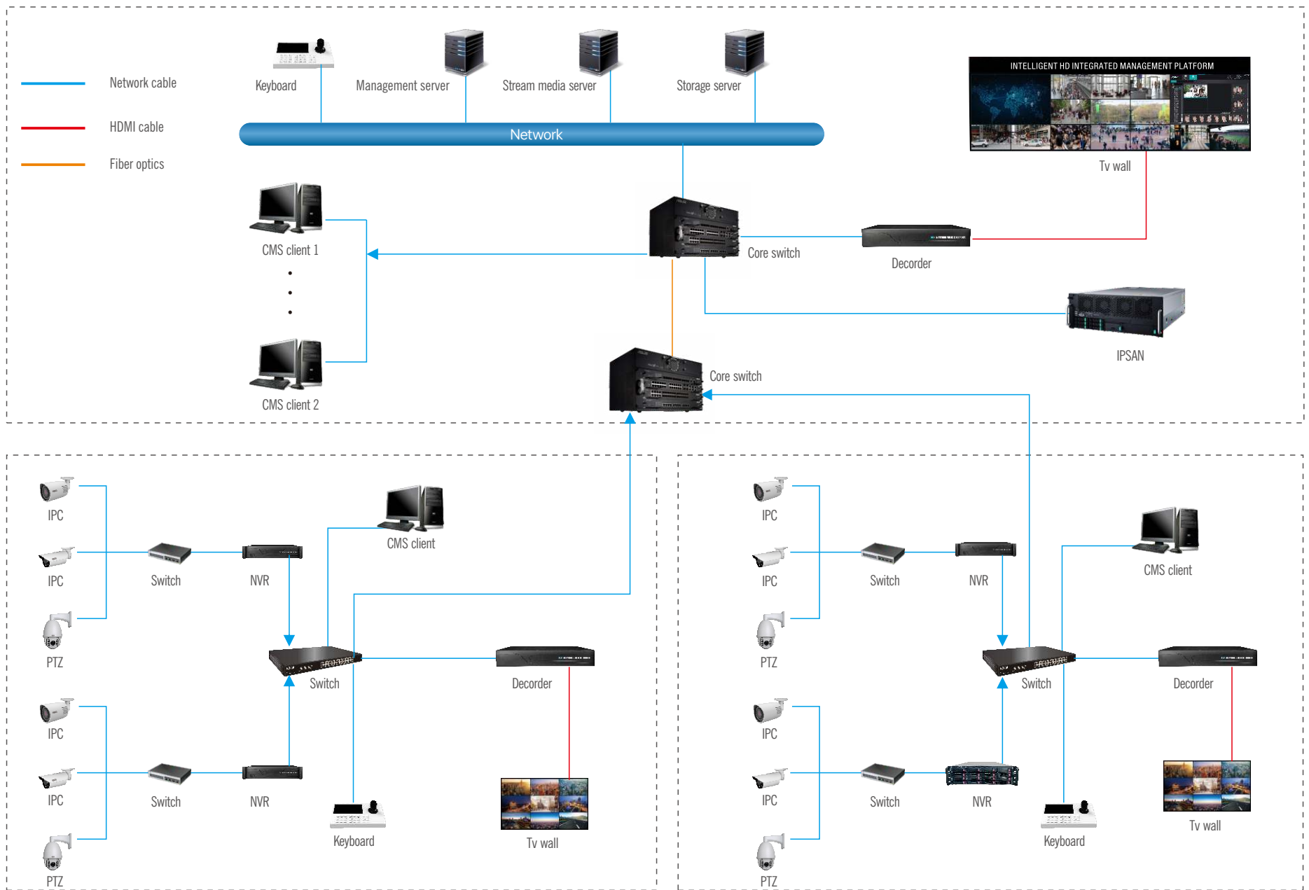
VIDEO SURVEILLANCE SYSTEM ARCHITECTURE
